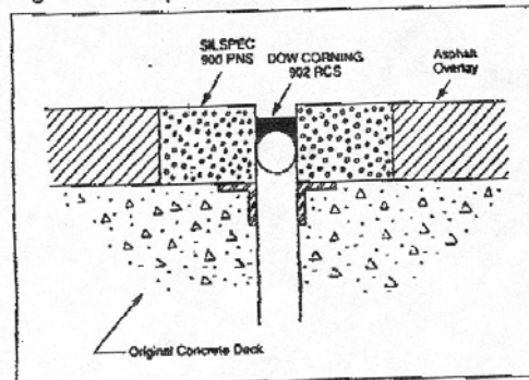
Figure 4 — Strip-Seal Repair
