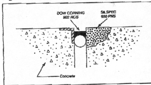
Figure 2 — New Construction "T" Joint Repair or Elastomeric Joint Repair
