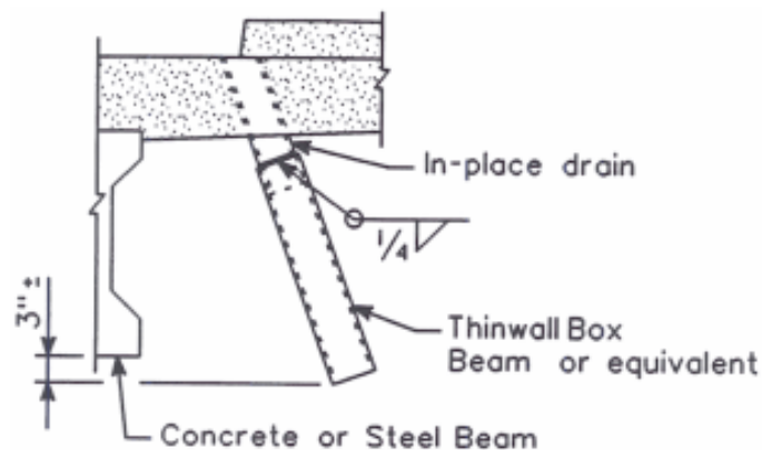
Exhibit X.35 Drain Extension
