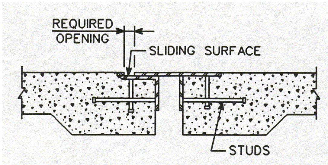
Exhibit X. 16 Plate Joint
